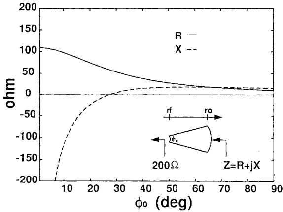
Fig. 3. The impedance of the sectorial component of the four-way power divider seen from the outer port versus the sector angle \phi_0 at frequency f_o = 3.3 GHz. The outer radius r_o is 26.6 mm.
